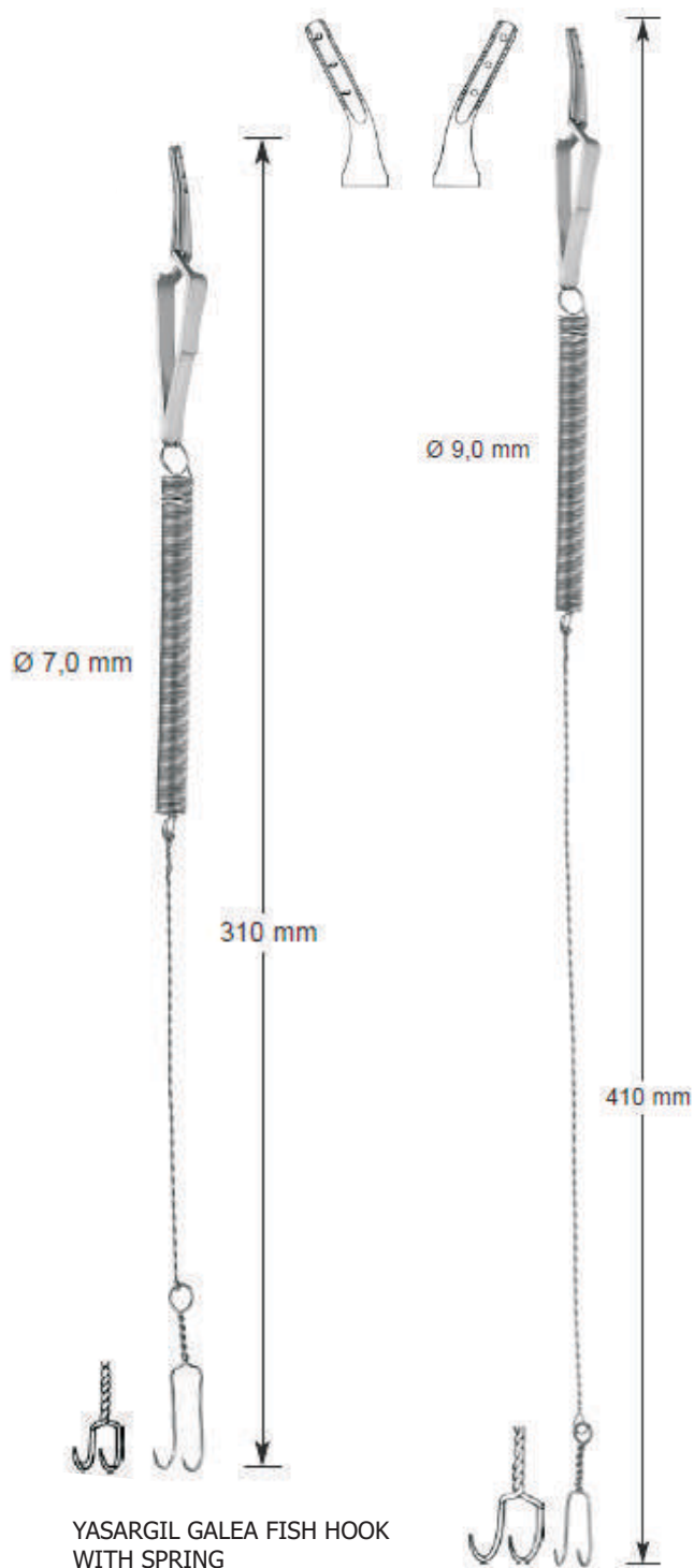
YASARGIL GALEA FISH HOOK WITH SPRING
